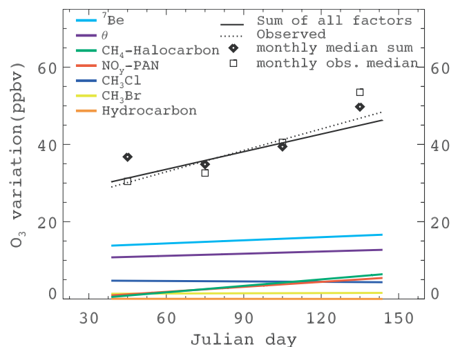
Figure 8. Same as Figure 4 but for high latitudes. The minimum \text{O}_3 concentration in the data set is 26 ppbv.
