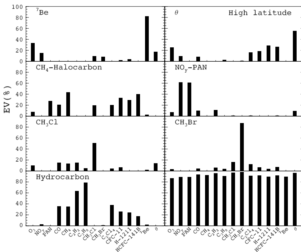
Figure 5. Same as Figure 1 but for high latitudes ( 60^{\circ} – 85^{\circ} N).
