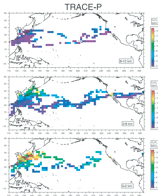
Figure 8. Same as Figure 5 but for \text{C}_2\text{Cl}_4 .
