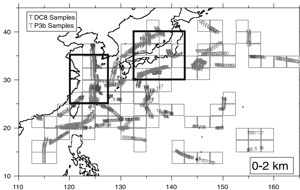
Figure 18. Location of all whole air samples collected between 0 and 2 km and west of 165°E on the NASA P-3B (light grey) and the NASA DC-8 (dark grey) during TRACE-P. The numbers represent flight number. The black boxes represent the “Japan Coast” (RHS) and “China Coast” (LHS) sample subsets.
