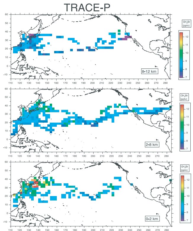
Figure 6. Same as Figure 5 but for \text{CH}_3\text{Br} .
