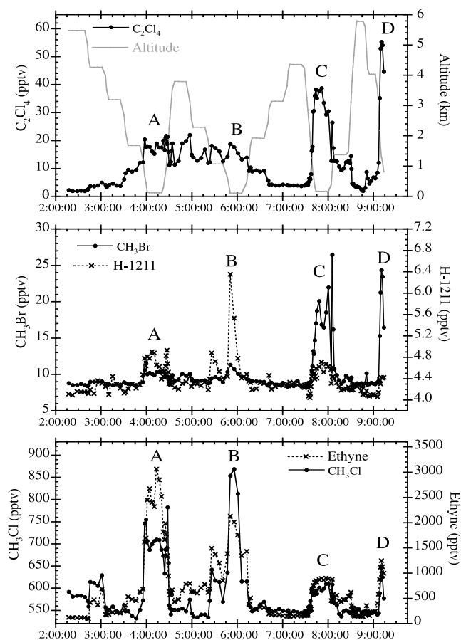
Figure 22. Mixing ratios of selected trace gases versus time for TRACE-P P-3B Flight 14 transit from Okinawa to Yokota, (near Tokyo). The different low altitude plumes are marked A–D.
