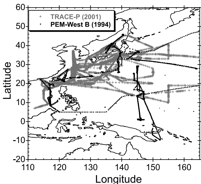
Figure 1. Whole air sample locations for PEM-West B and TRACE-P.
