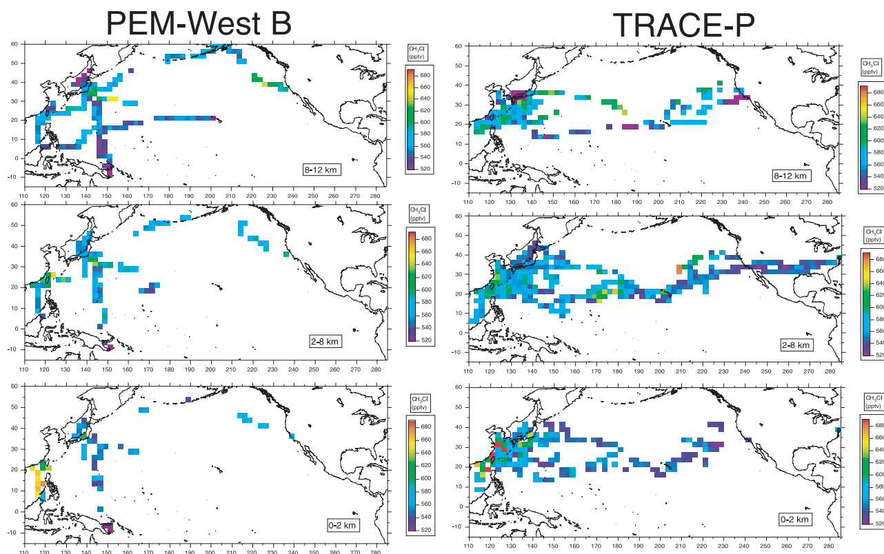
Figure 4. Same as Figure 3 but for \text{CH}_3\text{Cl} .
