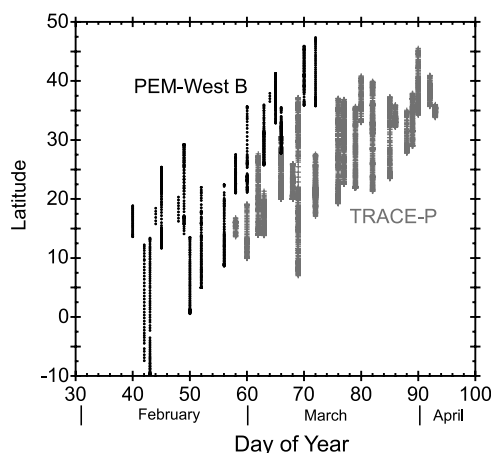
Figure 10. Temporal distribution for whole air samples collected west of 165^{\circ}\text{E} during PEM-West B and TRACE-P.
