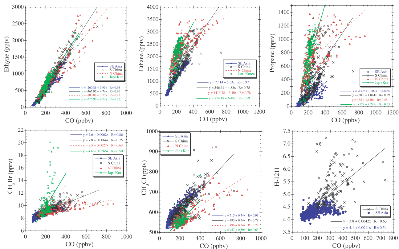
Figure 21. Selected trace gas mixing ratios versus CO for classifications SE Asia, South China, North China, and Japan + Korea as shown in Figure 20 (and see text). Note: The top 5% of data have been removed to better represent regional averages.
