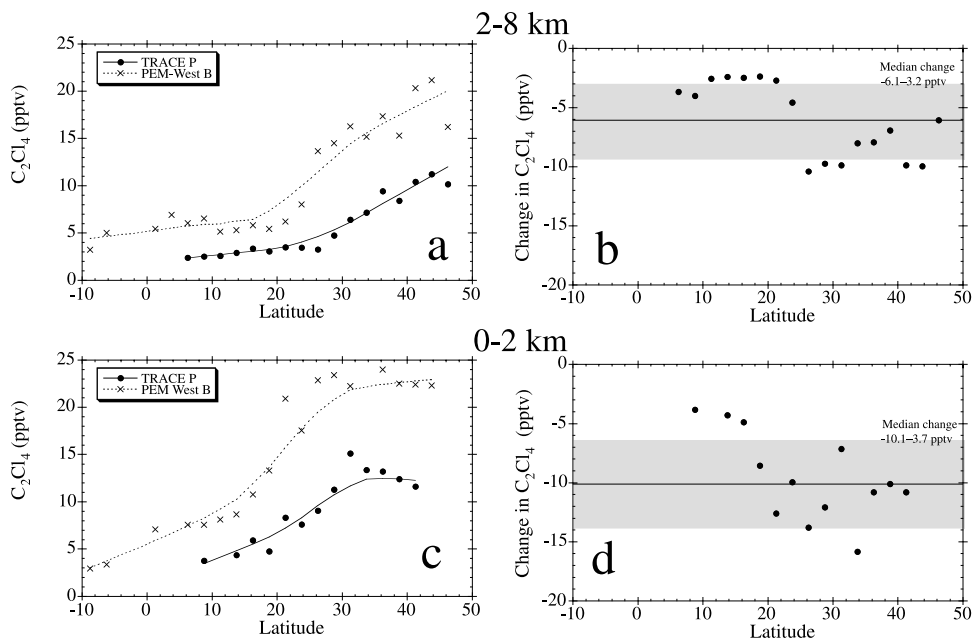
Figure 15. Same as Figure 12 but for C_2Cl_4 .
