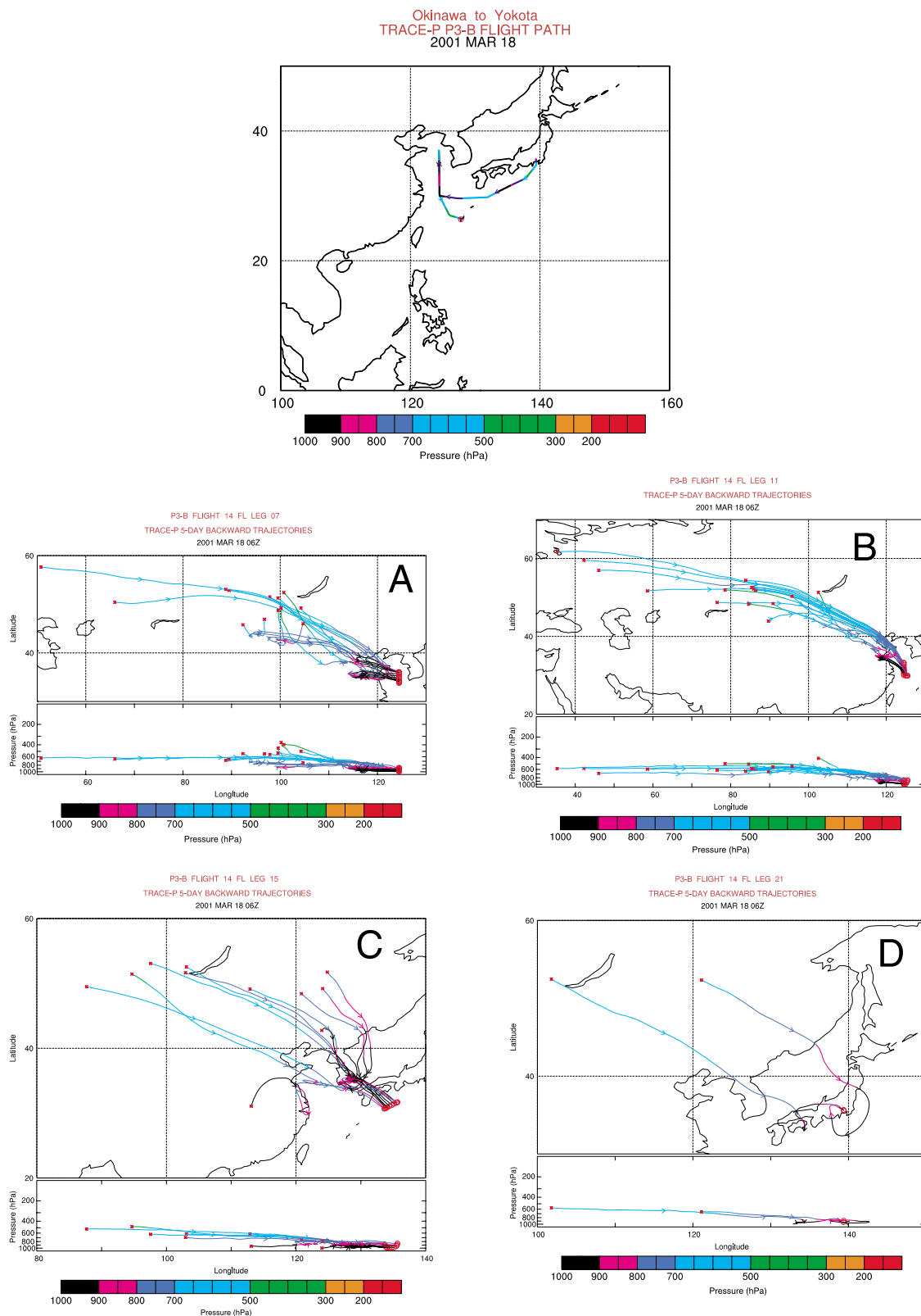
Figure 23. Flight track and backward trajectories for TRACE-P P-3B Flight 14. The different low altitude plumes are marked A–D as in Figure 22.
