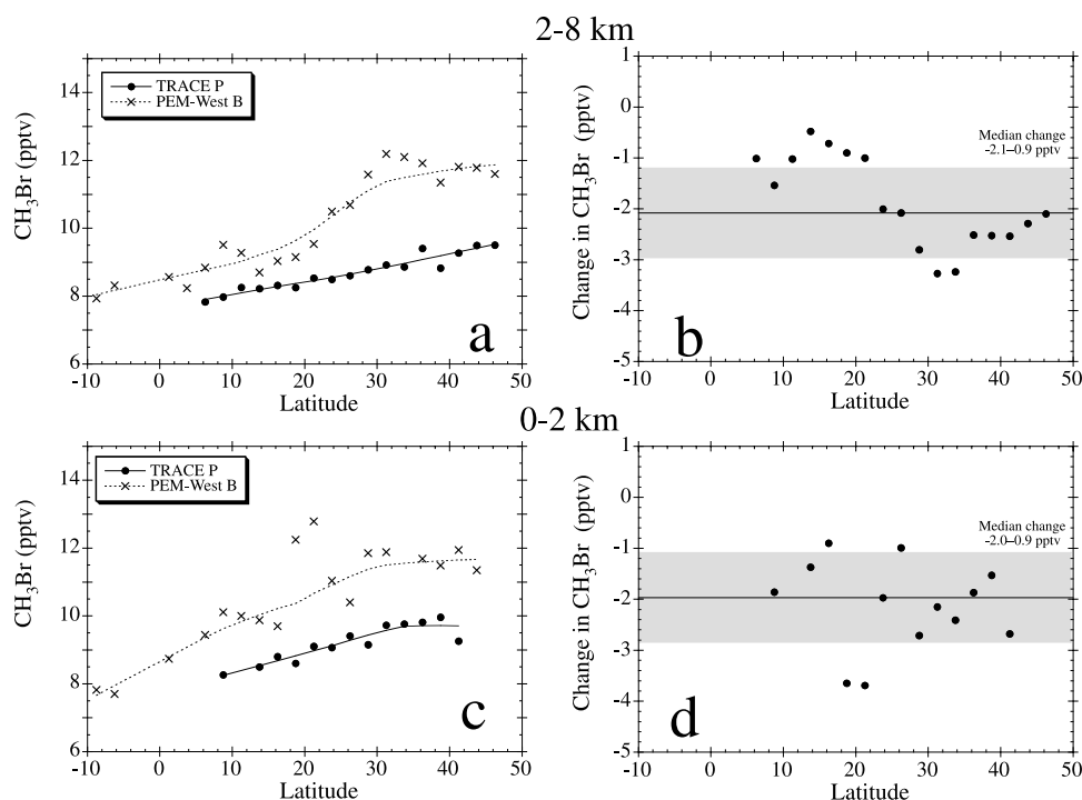
Figure 17. Same as Figure 12 but for \text{CH}_3\text{Br} .
