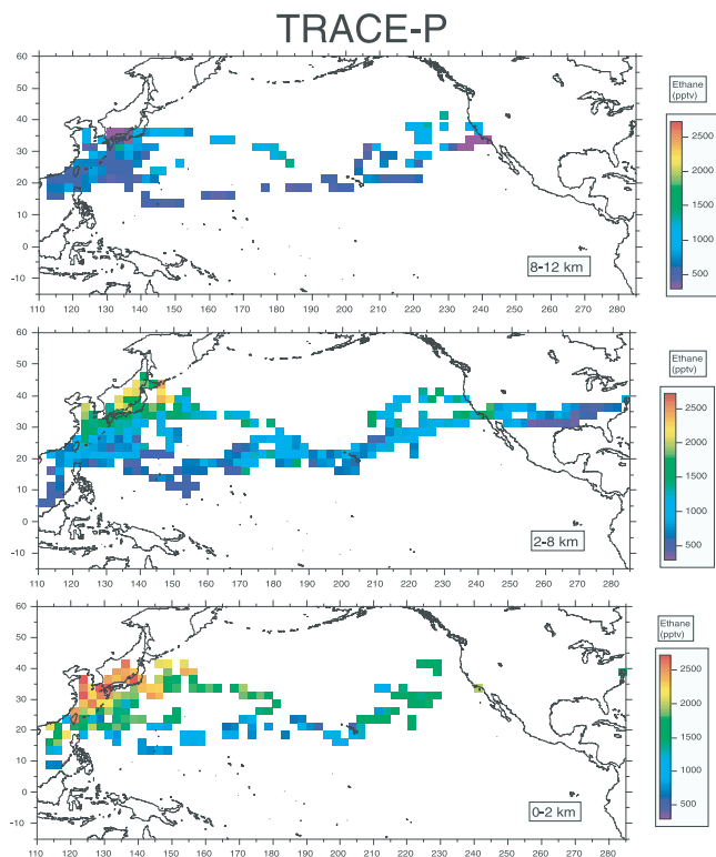
Figure 5. Regional distributions of ethane during TRACE-P illustrated as 2.5^\circ \times 2.5^\circ latitude/longitude patches color-coded by average mixing ratio. The data are divided into three altitude ranges representing the lower (0–2 km), middle (2–8 km) and upper (8–12 km) troposphere.
