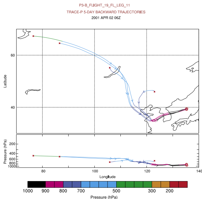
Figure 24. Backward trajectory for a low altitude air mass containing methyl bromide mixing ratios of nearly 35 pptv encountered during TRACE-P P-3B Flight 19, which was a Yokota local flight over the Sea of Japan.
