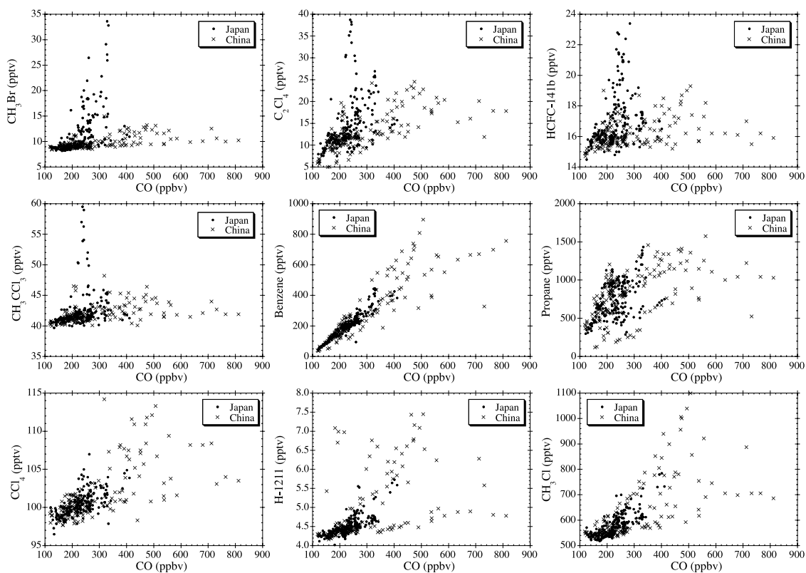
Figure 19. Correlation versus CO for samples collected near the coast of Japan (30–40°N, 135–142.5°E with landing samples removed) and off the coast of China (25–35°N, 120–127.5°E) as shown in Figure 18.
