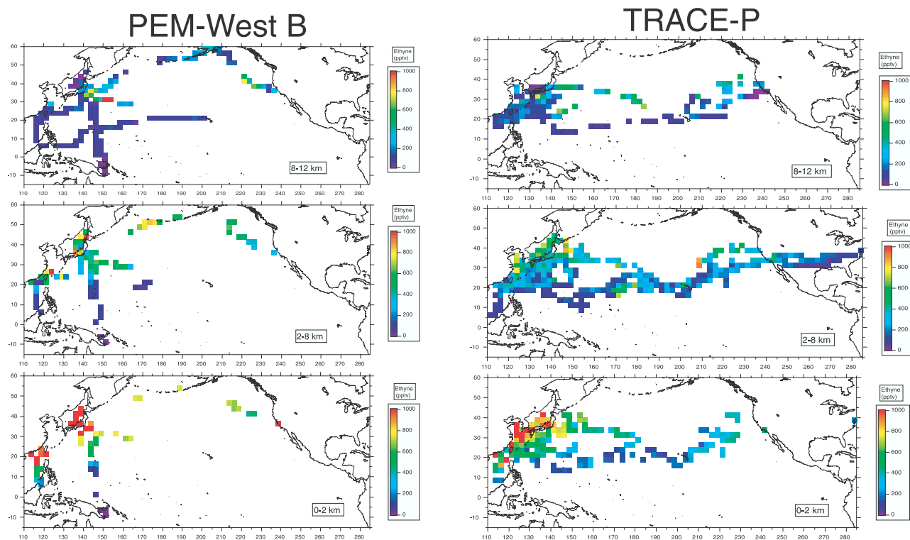
Figure 3. Same as Figure 3 but for ethyne.
