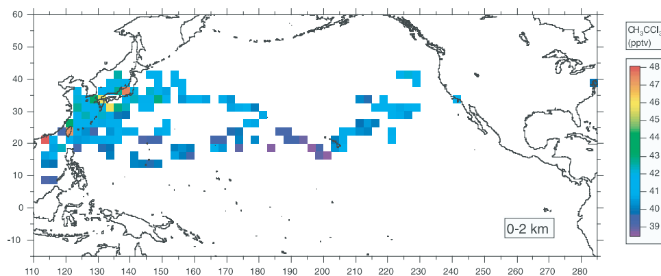
Figure 13. Low-altitude (0–2 km) regional distributions of \text{CH}_3\text{CCl}_3 during TRACE-P illustrated as 2.5^\circ \times 2.5^\circ latitude/longitude patches color-coded by average mixing ratio.
