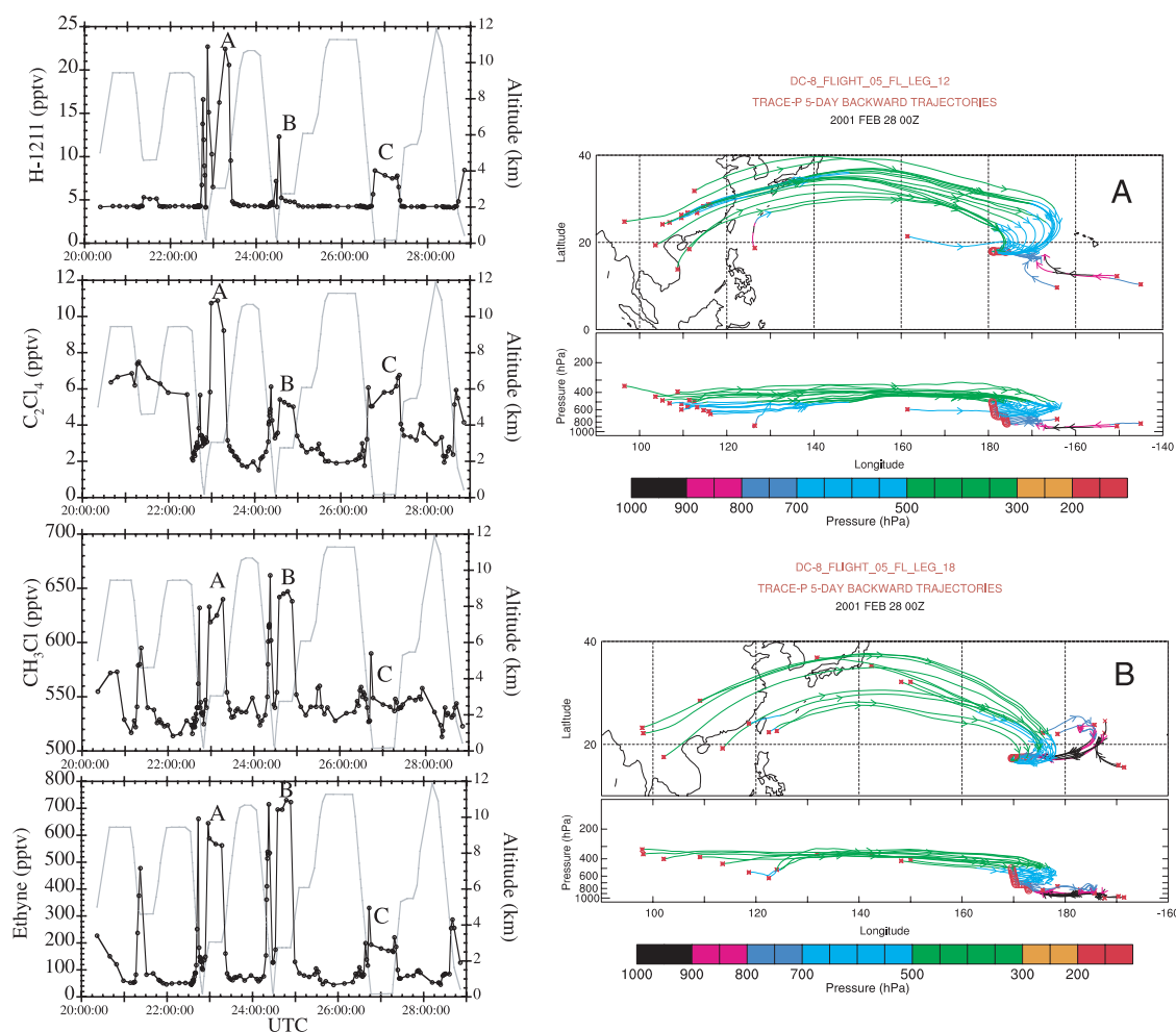
Figure 25. Mixing ratios of selected trace gases and altitude versus time for TRACE-P DC-8 Flight 5. Very high Halon-1211 was observed in plume A, which had a backward trajectory from mixed regions of China. Lower Halon-1211 mixing ratios were observed in plume B, with its backward trajectory potentially showing a greater biomass burning influence from further west.
