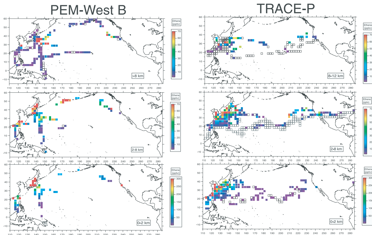
Figure 2. Regional distributions of ethene during PEM-West B and TRACE-P illustrated as 2.5^\circ \times 2.5^\circ latitude/longitude patches color-coded by average mixing ratio. Average mixing ratios below detection limit are shown as open squares. The data are divided into three altitude ranges 0–2 km, 2–8 km, and 8–12 km.
