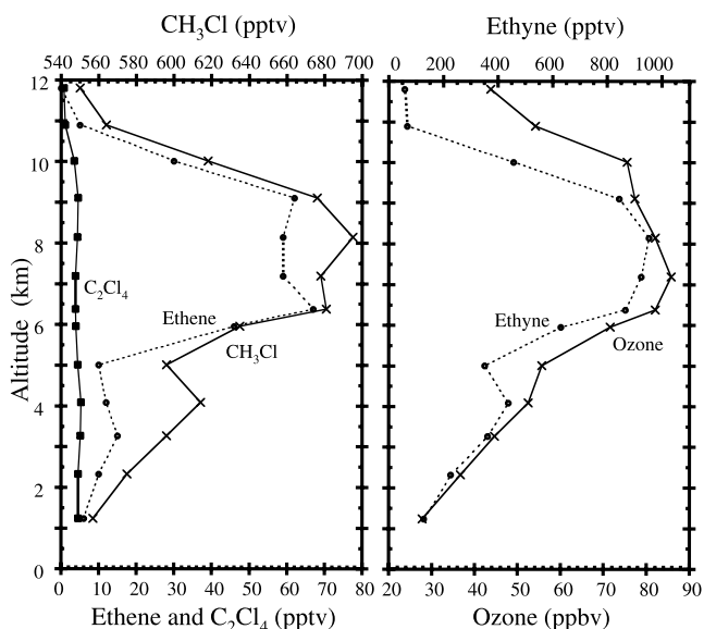
Figure 26. Vertical profile from TRACE-P DC-8 Flight 4, a biomass burning plume in the mid troposphere NE of the Hawaiian Islands.
