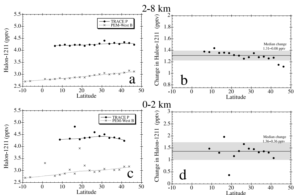
Figure 12. Median mixing ratios of Halon-1211 for 2.5^\circ bins for TRACE-P and PEM-West B over the western Pacific (west of 165^\circ\text{E} ) for the altitude ranges (a) 2–8 km (c) 0–2 km. Figure 12b and 12d show the difference between the median data in Figures 12a and 12c, respectively, for the two missions (TRACE-P - PEM-West B). The line is the mean difference over all latitudes and the shaded band is the 1 standard deviation uncertainty.
