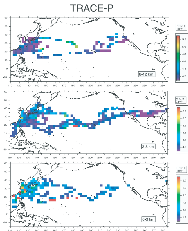
Figure 7. Same as Figure 5 but for Halon-1211.
