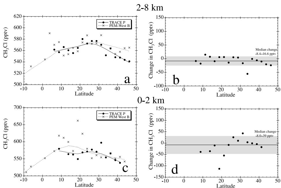
Figure 16. Same as Figure 12 but for CH_3Cl .
