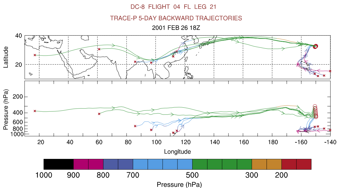
Figure 27. Backward trajectories for the vertical profile in Figure 26.
