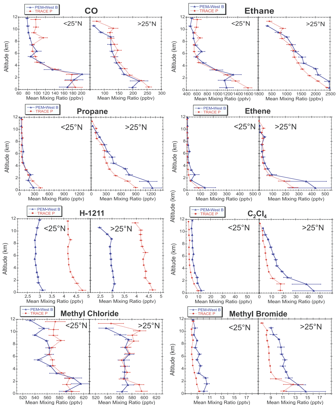
Figure 9. Mean mixing ratios of selected trace gases for 1-km altitude increments for all samples collected west of 165°E for PEM-West B (blue) and TRACE-P (red). Error bars are the 95% confidence level of the mean.
