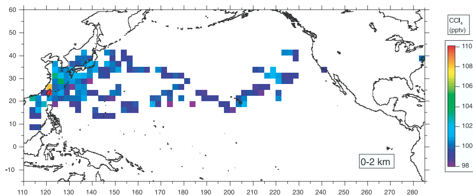
Figure 14. Same as Figure 13 but for \text{CCl}_4 .
