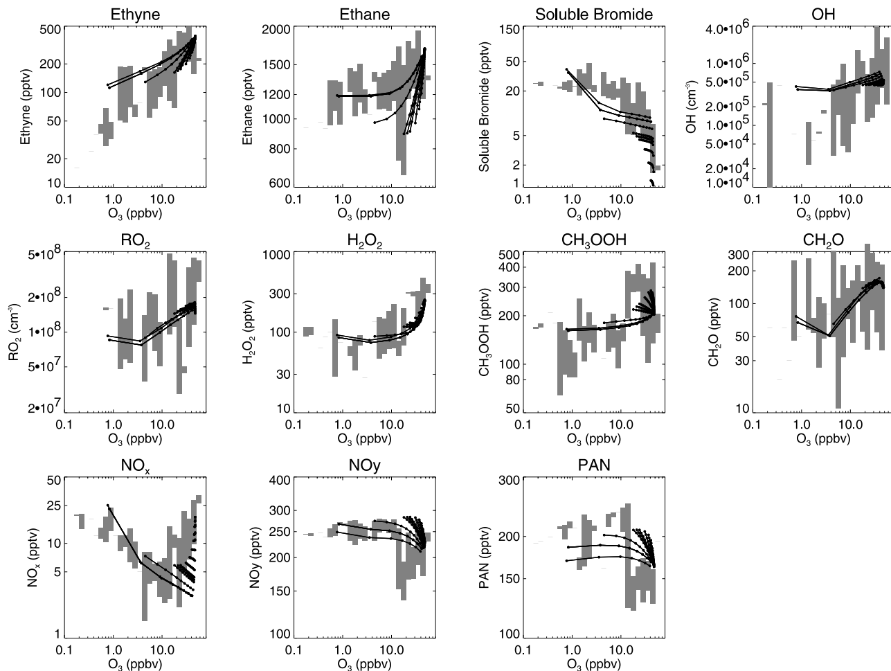
Figure 5. Chemical evolution during O 3 depletion events in the Arctic boundary layer in spring, plotted against the O 3 chemical coordinate. Aircraft measurements from TOPSE (north of 50°N, below 500 m altitude, March 23–May 22, 11:00–13:00 local time) are shown as grey bars ( \pm 1 standard deviation). Model results (section 3) are shown as lines for different initial bromide concentrations (0 to 43 pptv): the higher the initial bromide concentration, the larger the O 3 loss and thus the longer the line. The model simulations were conducted for 10 days starting at noon, and noontime concentrations are shown here (symbols on lines). See Table 1 for definitions of the lumped species.
