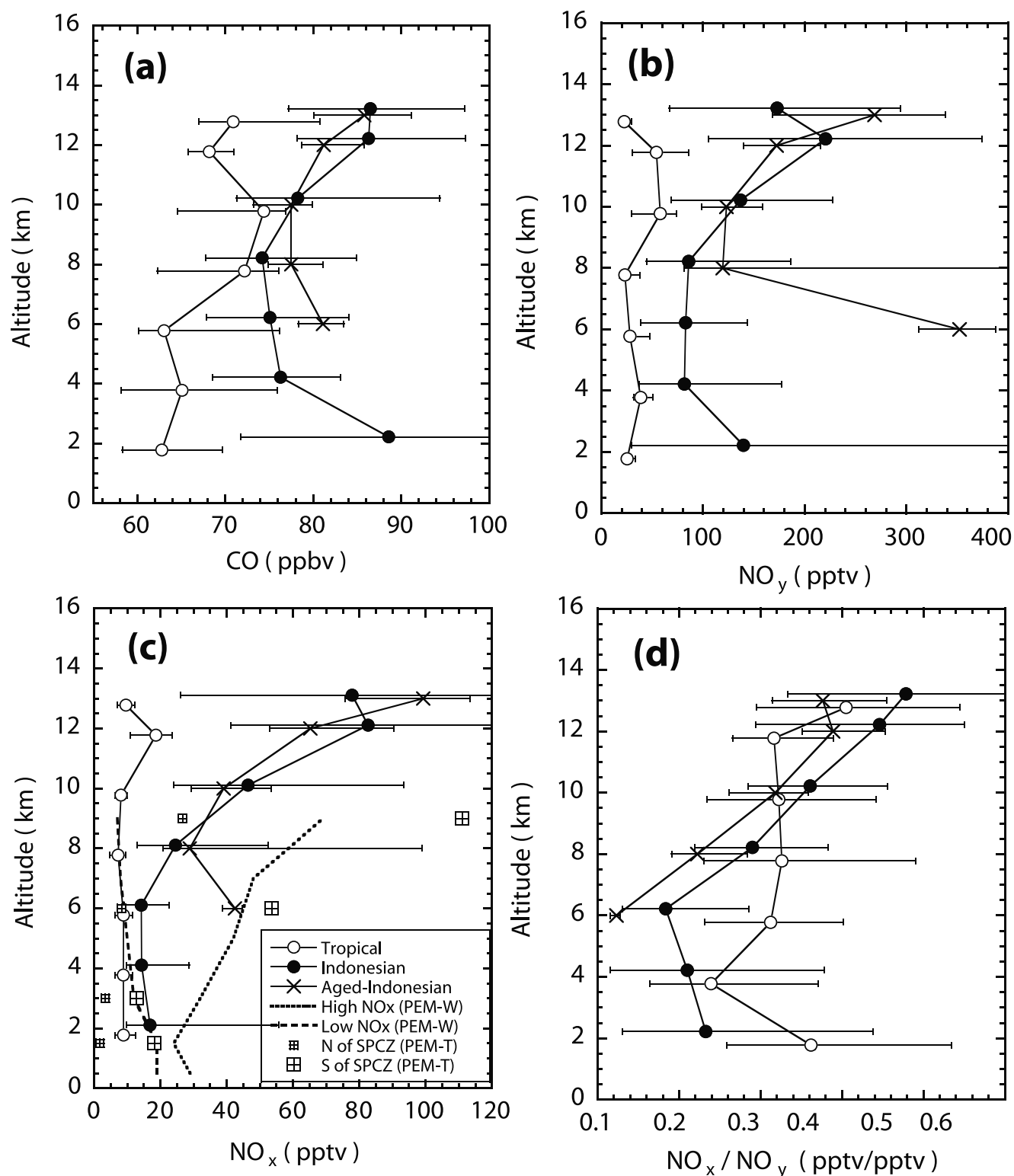
Figure 3. Vertical profile of the median values of the CO, NO y , NO x , and NO x /NO y ratio in Indonesian, tropical, and aged Indonesian air masses. The bars indicate the central 67% range. In Figure 3c, values obtained during the PEM-West B (PEM-W) and PEM-Tropics A (PEM-T, values of NO instead of NO x ) experiments are also shown.
