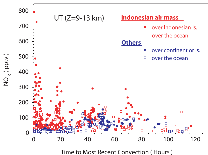
Figure 12. The NO x mixing ratio as a function of the time difference between the measurement and most recent encounter with a deep convection. All the data obtained in the UT at latitudes south of 10°N are shown.
