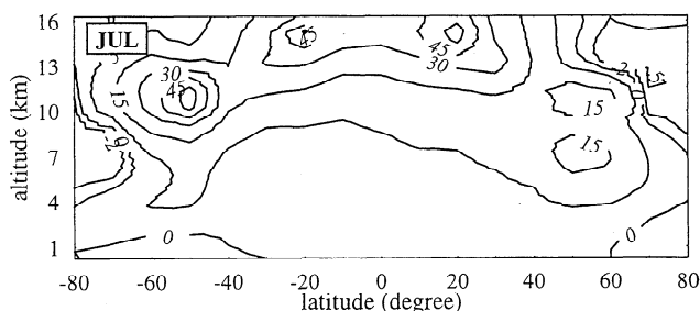
Figure 4. Calculated percent changes in diurnally averaged OH concentration for the month of July due to inclusion of convective transport to photochemical scheme PC1.
