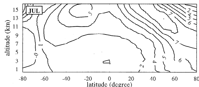
Figure 6. Calculated percent changes in diurnally averaged OH concentration for the month of July due to inclusion of soil sinks of CO and \text{CH}_4 to photochemical scheme PC1.
