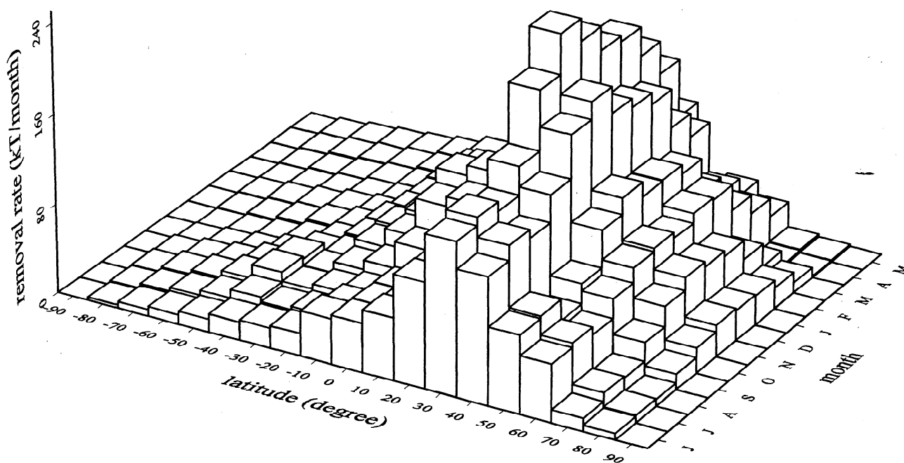
Figure 7. Latitude-time cross section of integrated monthly surface removal rates of C_2H_6 per 10^\circ bin in steady state calculated using scheme PC3 and its surface observations.
