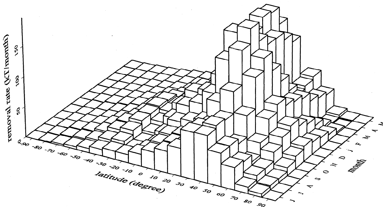
Figure 8. Latitude-time cross section of integrated monthly surface removal rates of C_3H_8 per 10^\circ bin in steady state calculated using scheme PC3 and its surface observations.
