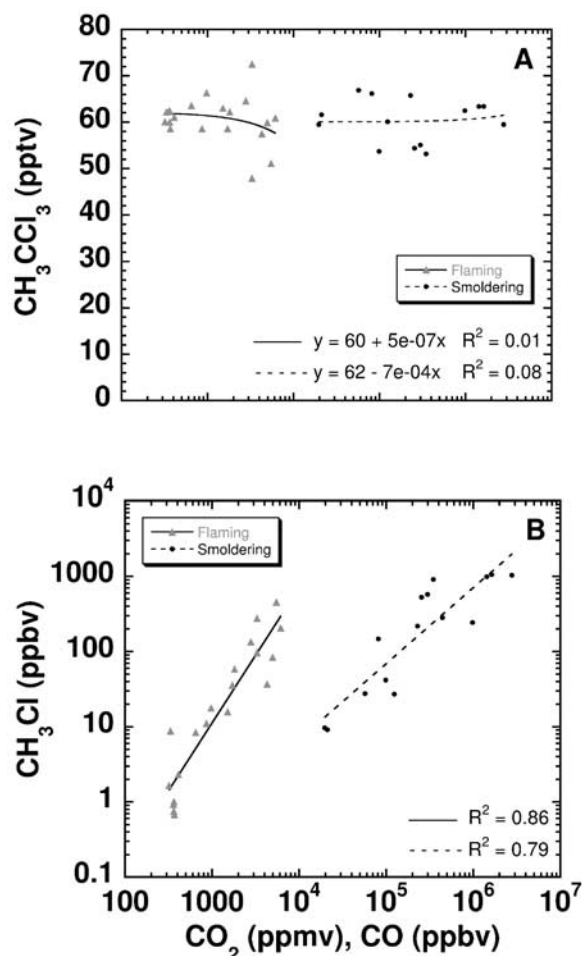
Figure 1. Scatter plots of ground-based air samples heavily impacted by savanna burning in northern Australia, Sep. 1999. (a) MCF vs. \text{CO}_2 during the flaming fire stage (triangles, n = 20 ) and vs. CO during smoldering (circles, n = 14 ); (b) \text{CH}_3\text{Cl} vs. \text{CO}_2 during flaming (triangles) and vs. CO during smoldering (circles). The equations displayed in Figure 1a are linear fits to the data. The fits in Figure 1b are linear fits to logarithmic data.
